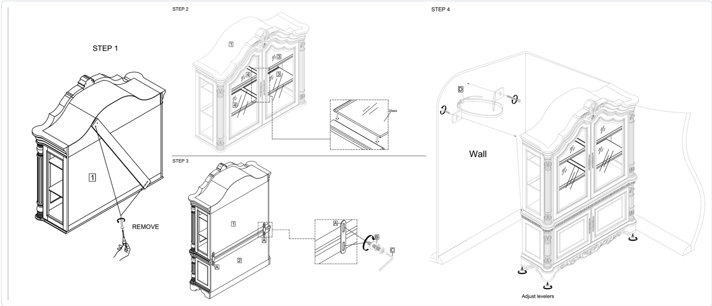
China base 42785862 / HMIS D8586-07 and china hutch 42885864 / HMIS D8586-08 (sheet pages 1-3)
