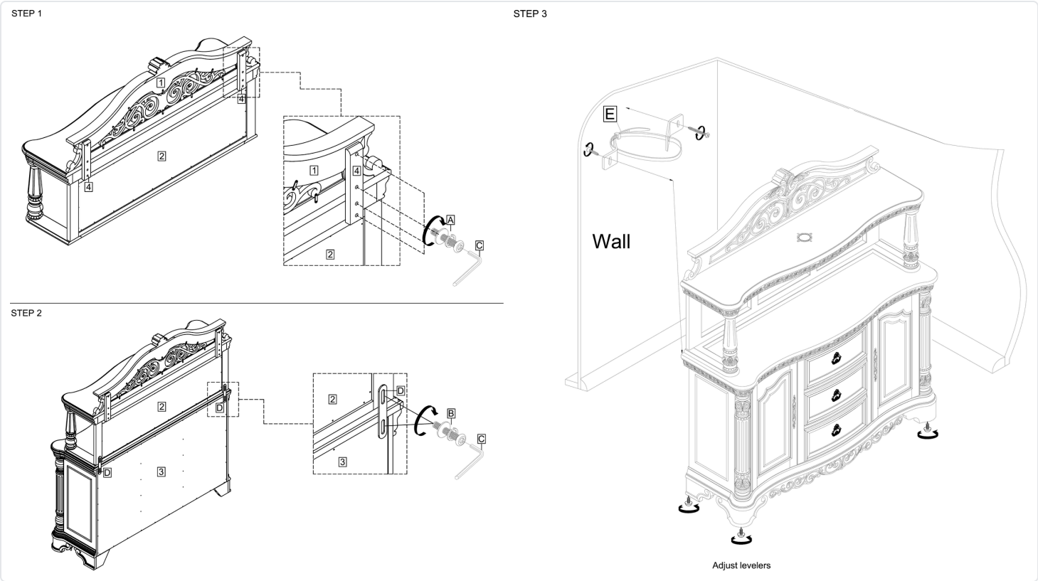
Server 42985866 / HMIS D8586-06 and server hutch 43785863 / HMIS D8586-10 (sheet pages 2-3)
