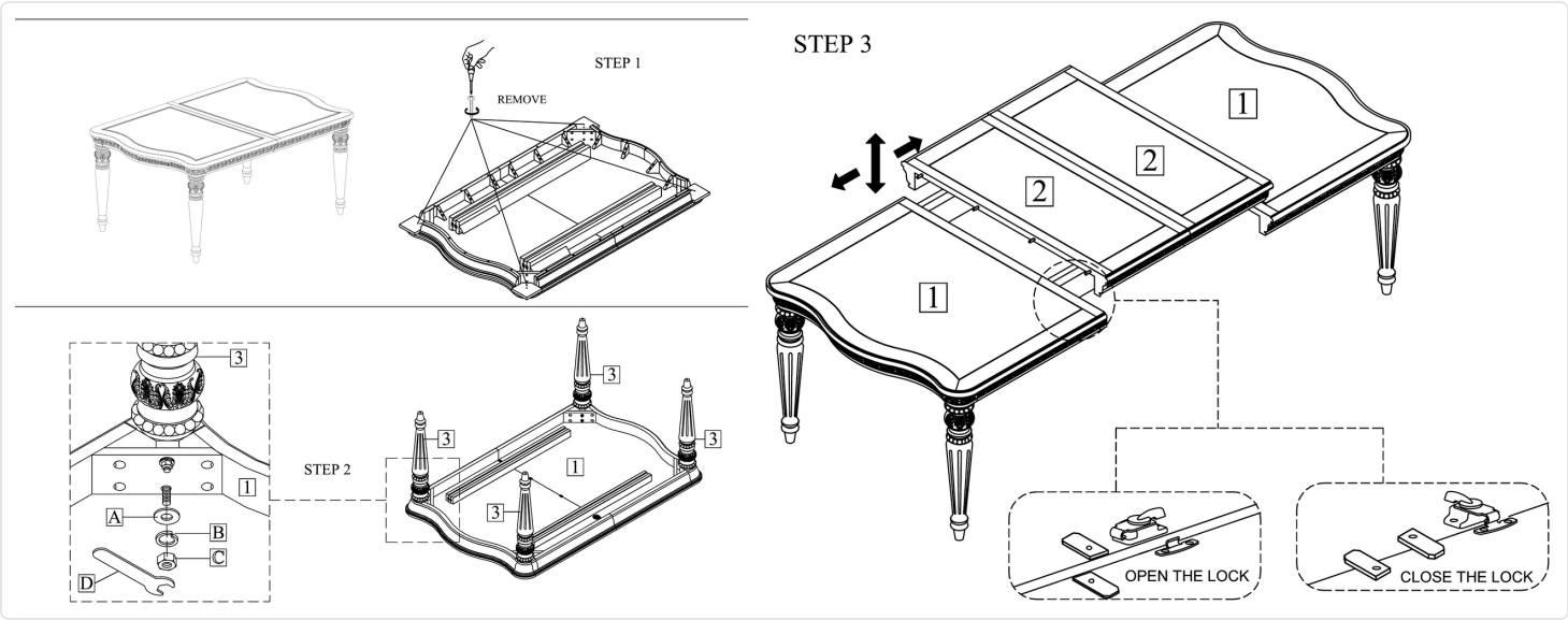
Rectangle dining table 42285862 / HMIS D8586-11 (sheet pages 1-2: legs, then leaves)
