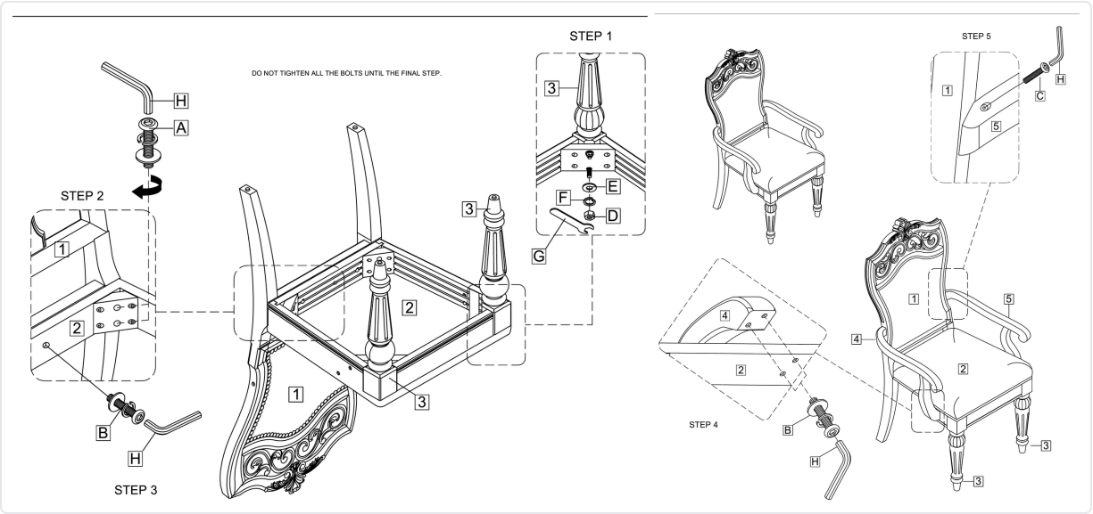
Upholstered arm chair 42685860 / HMIS D8586-04 (sheet pages 1-2)
