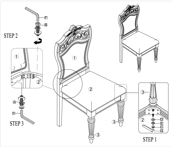
Upholstered side chair 42485866 / HMIS D8586-03
